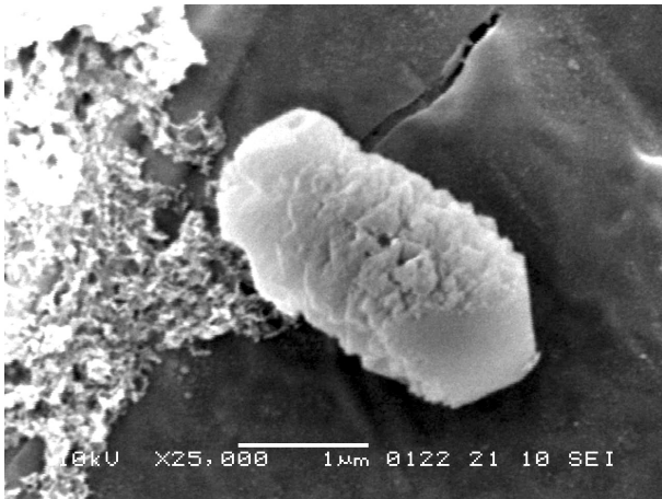
Fig. 3: SEM picture of isolated microcrystal on a Formvar-covered TEM grid. Notice the multilayered structure and sharpened extremities. Sketch of two (001)T type texture, with or without rotation.
